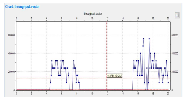
Figure 4: Throughput vector graph of two Hosts when Obstacles between them.
